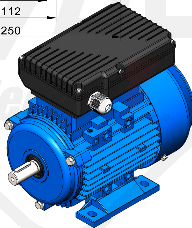
1ALJ-71-B3 Mounting diagram
