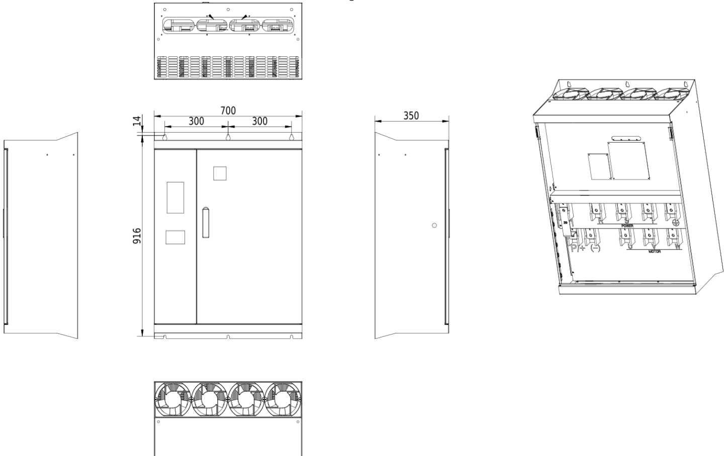
Dimensional drawing V810 - 280kW 4T2800
