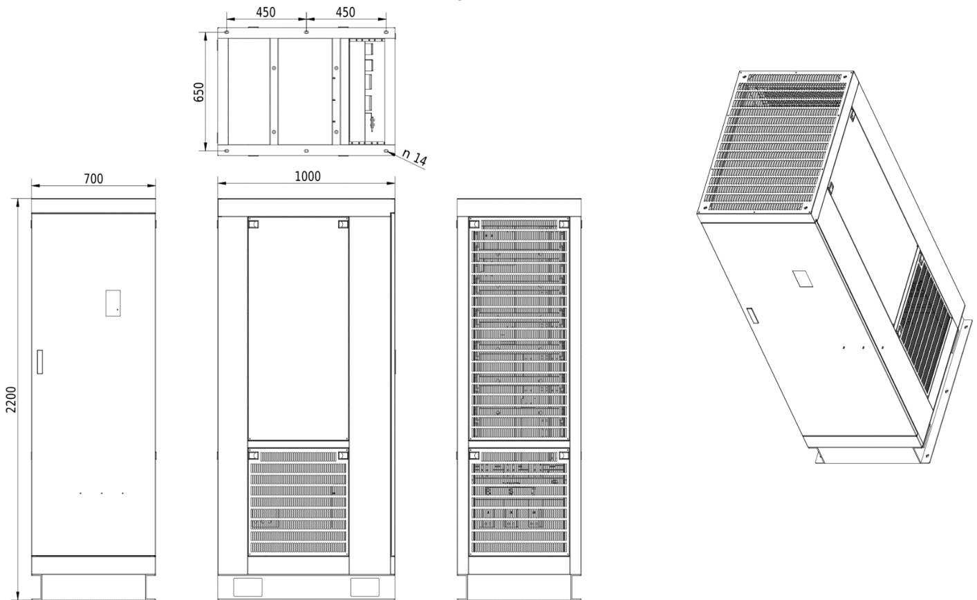
Dimensional drawing V810 - 1000kW 4T10000
